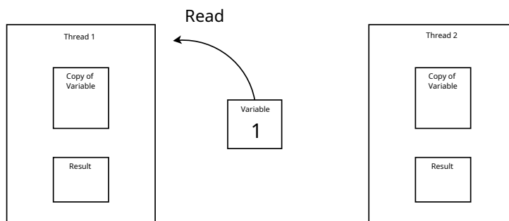
Figure 115: Thread 1 reads the variable
